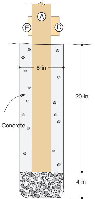
DRAWING 1b Optional Footing Detail
