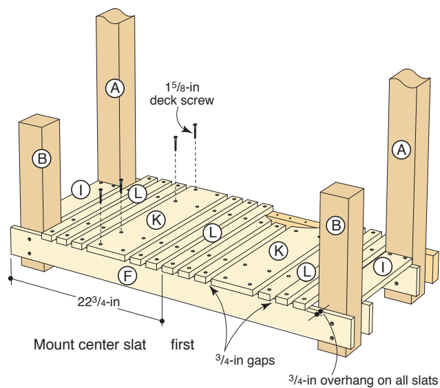
DRAWING 5 Lower slats
