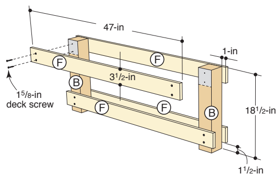
DRAWING 3 Front Assembly
