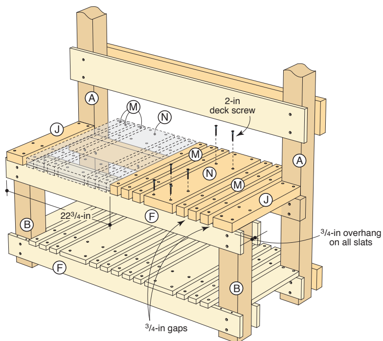
DRAWING 6 Seat slats
