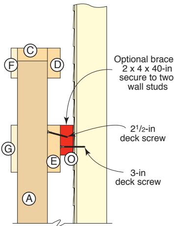
DRAWING 1a Optional House Connection
