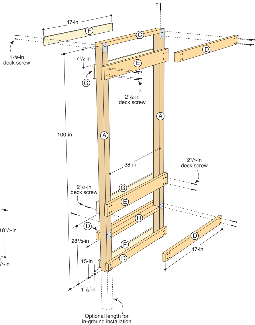
DRAWING 2 Back Assembly
