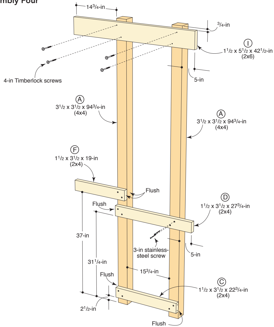
DRAWING 4 Leg Assembly Four
