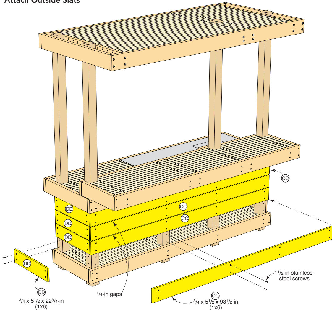
DRAWING 12 Attach Outside Slats
