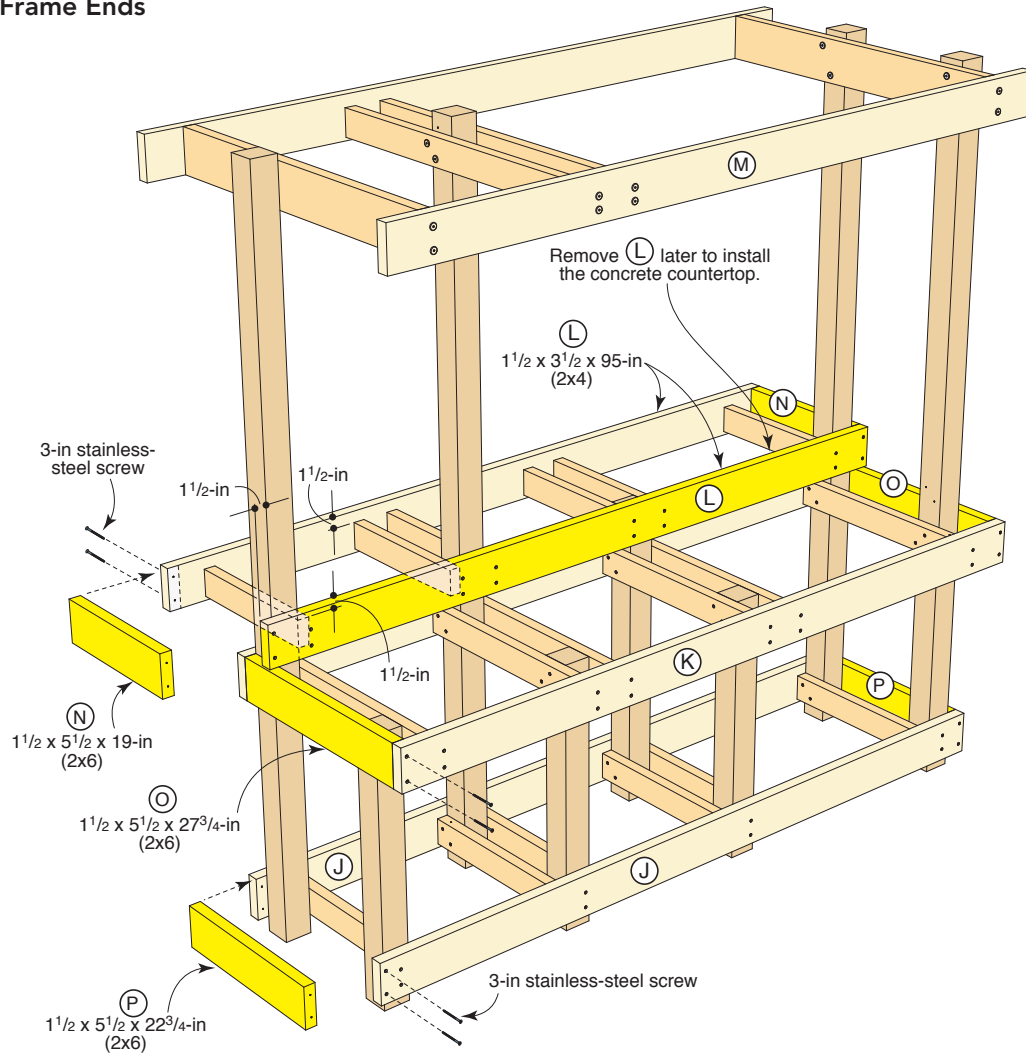
DRAWING 7 Frame Ends
