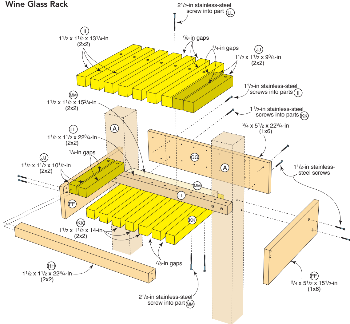
DRAWING 13 Wine Glass Rack
