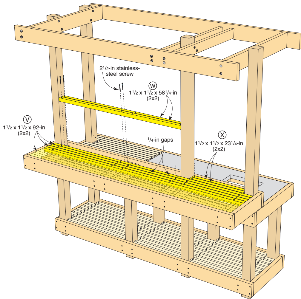
DRAWING 10 Bar Installation
