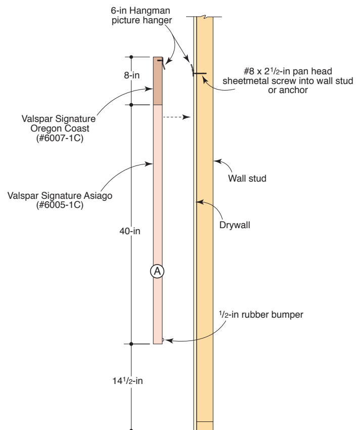
DRAWING 7 Optional Headboard Installation
