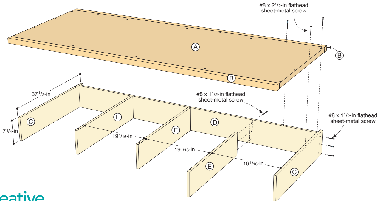
DRAWING 4 Top Assembly
