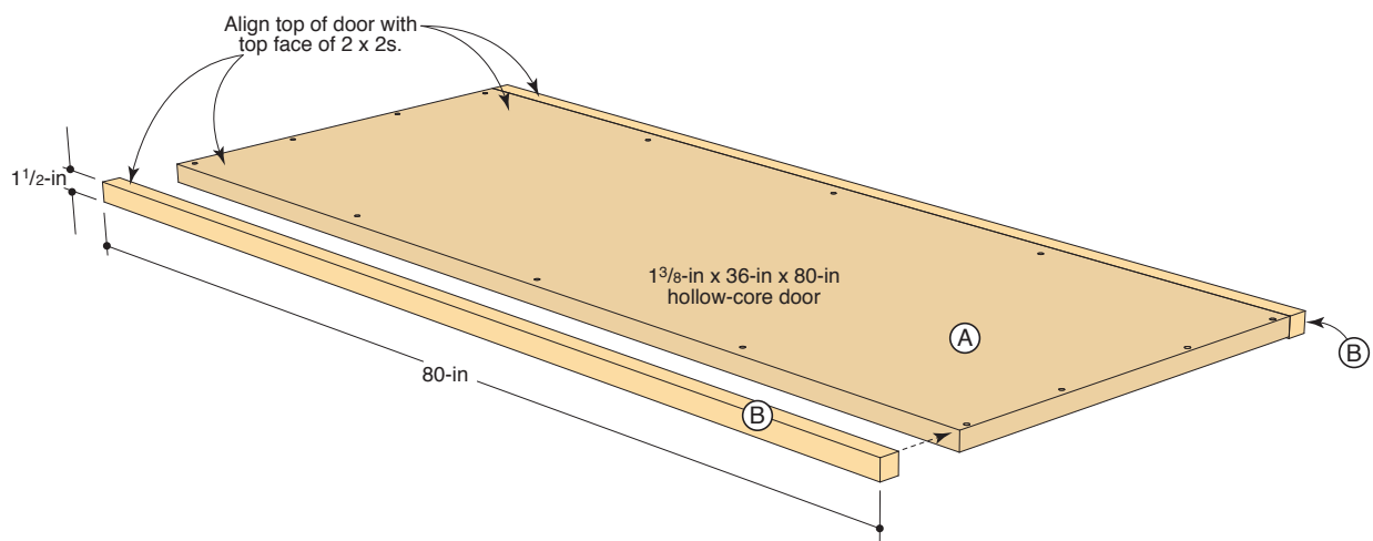
DRAWING 1 Top and Bottom
