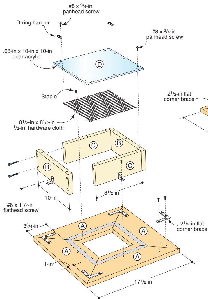
DRAWING 1 Small Planter
