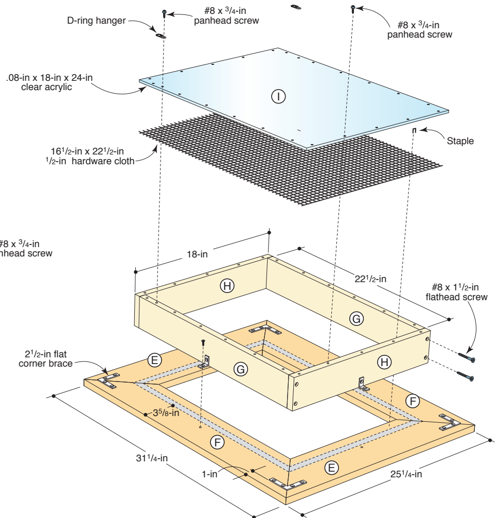
DRAWING 2 Large Planter
