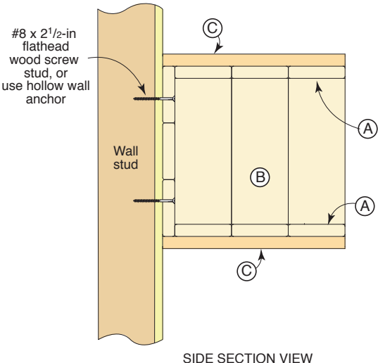
SIDE SECTION VIEW
