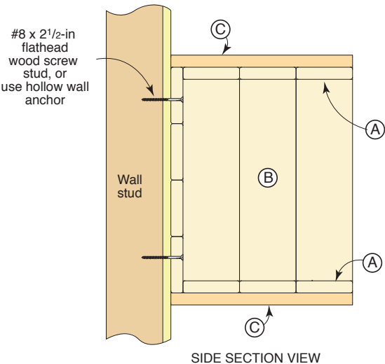
DRAWING 3 Wall Mounting Detail
