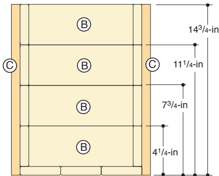
DRAWING 1 Cleat Length
