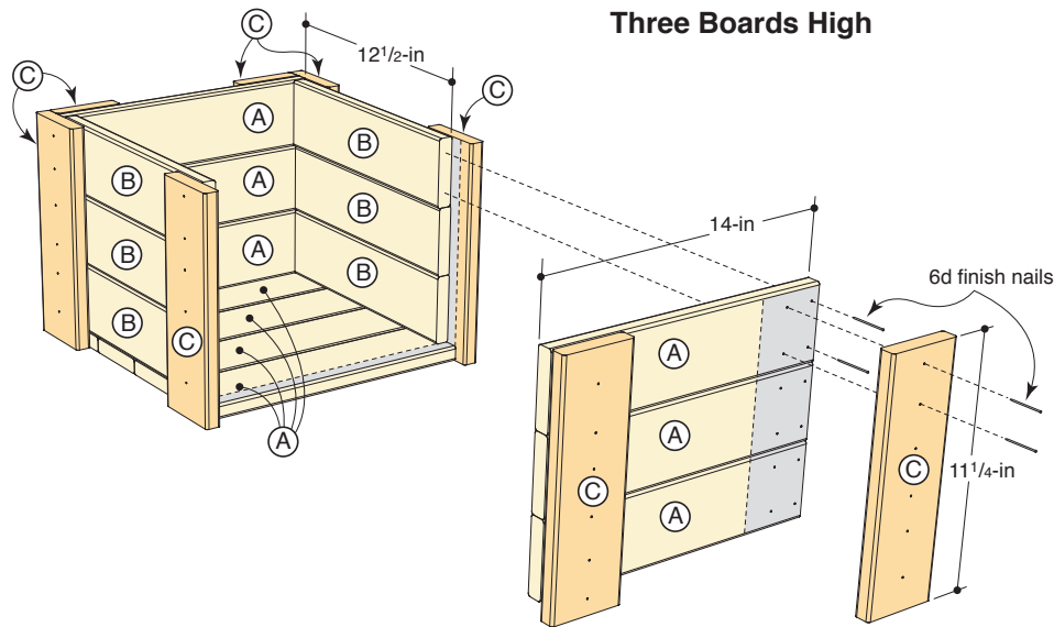
DRAWING 1 Cleat Length
