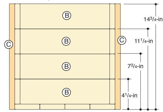
DRAWING 1 Cleat Length
