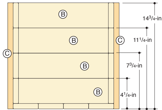
DRAWING 1 Cleat Length
