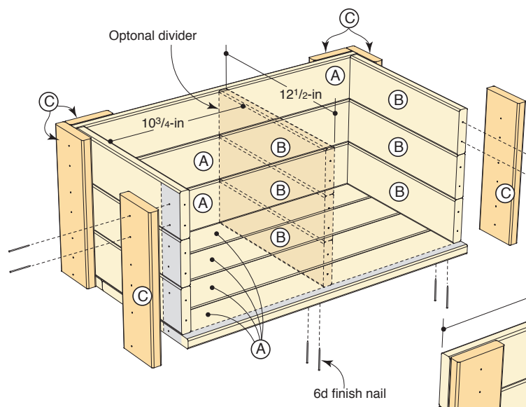
DRAWING 1 Cleat Length
