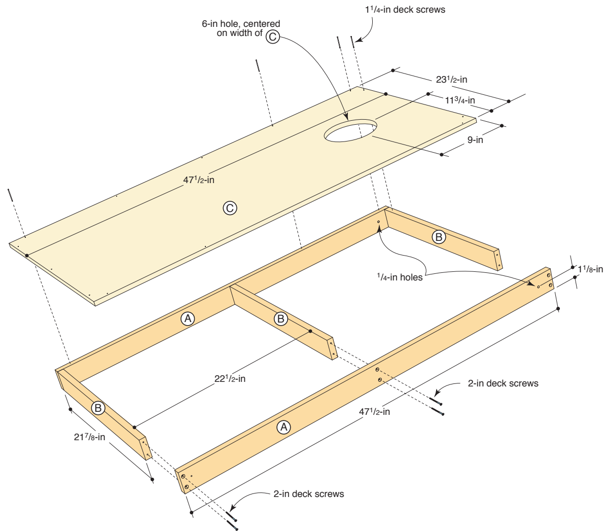
DRAWING 1 Top Assembly
